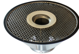
Cone for Interceptors - Included
