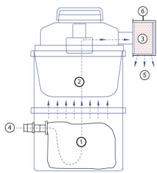
CR-1000 (SS) Series Air Flow Schematic
